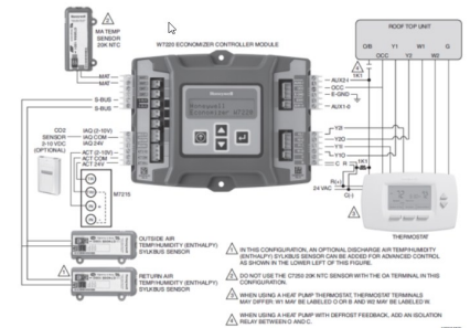
Fig. 4. Economizer with Sylix Bus sensors for enthalpy configuration with Honeywell W7215 black motor.
